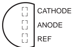
TL431, TL431A . . . LP PACKAGE (TOP VIEW)
