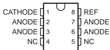
TL431, TL431A . . . D PACKAGE (TOP VIEW)
