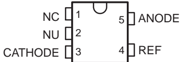
TL431, TL431A . . . DBV PACKAGE (TOP VIEW)
