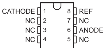
TL431, TL431A . . . P, PS, OR PW PACKAGE (TOP VIEW)
