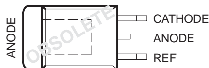
TL431 . . . KTP PACKAGE (TOP VIEW)
