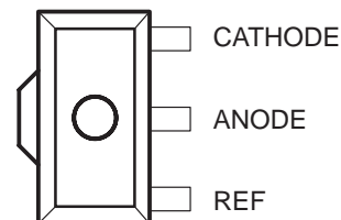
TL431 . . . PK PACKAGE (TOP VIEW)
